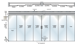
Telescopic Synchro Sliding 3 Fix + 3 Sliding Doors
